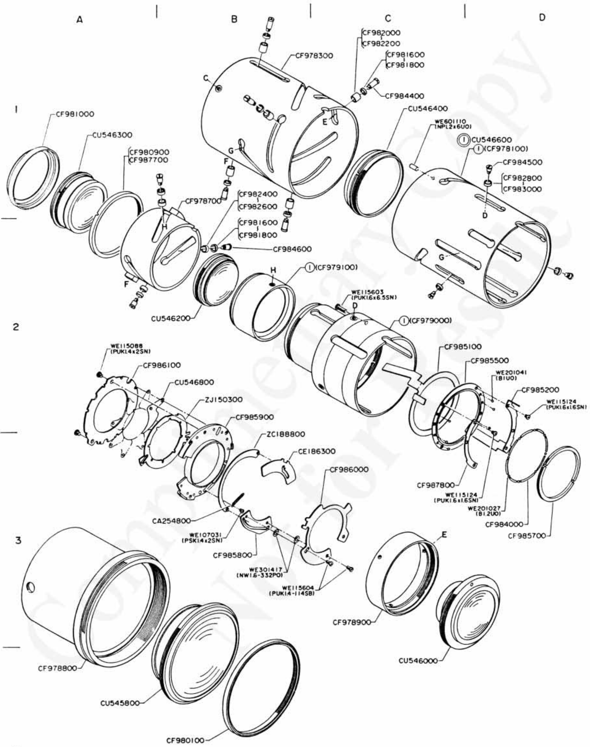
4 EXPLODED PARTS DIAGRAM
