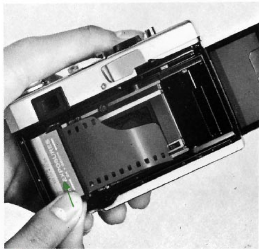
3 Insert film magazine onto rewind shaft.
